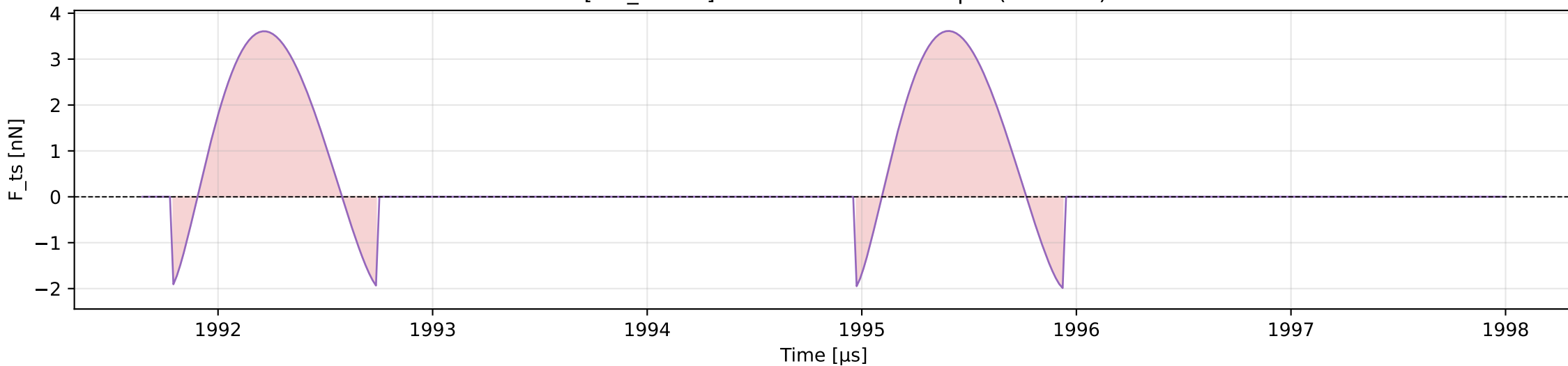
W3 [tail_stable] 1991.648-1998.000 \mu\text{s} (override)
